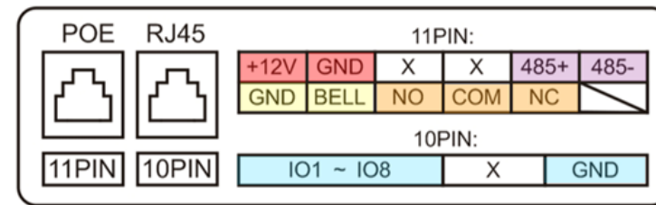
Figure 1.2-1 C313X interface
